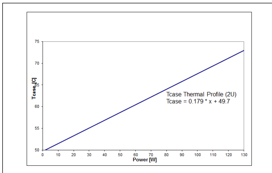
Figure 5-19. Tcase: 4-Core 130W Thermal Profile 2U
