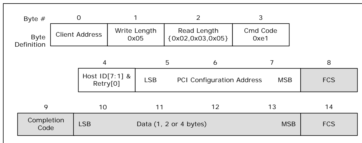
Figure 2-47. RdPCIconfigLocal()
