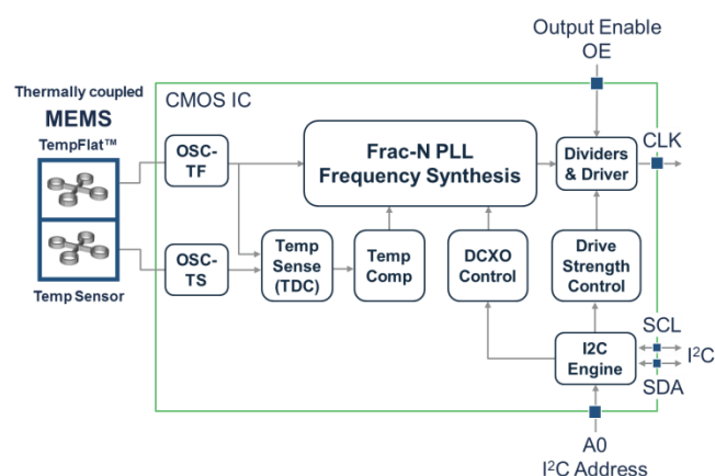
Figure 38. Block Diagram
