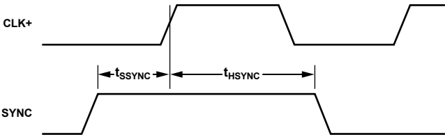
Figure 3. SYNC Timing Inputs
