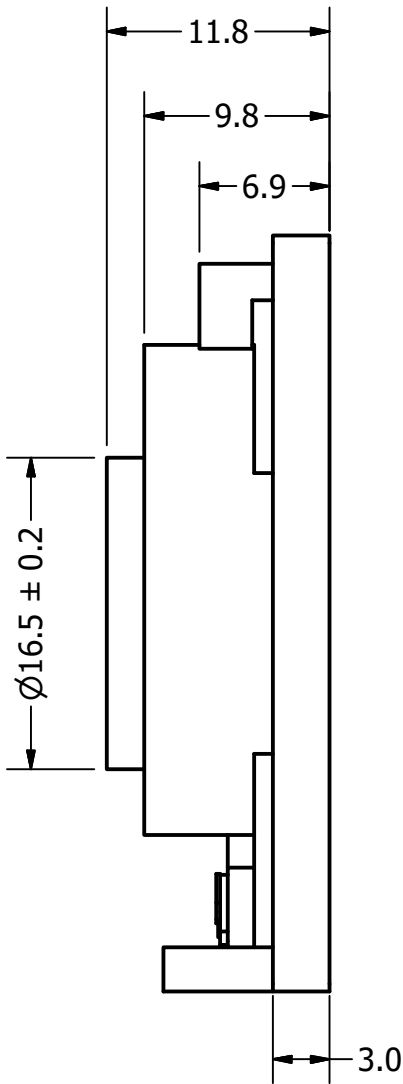
Side View
