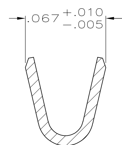
SECTION Y-Y WIRE BARREL SCALE 20:1
