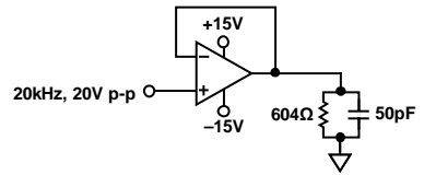
Figure 28. Output Swing, VS = ±15V, G = +1
