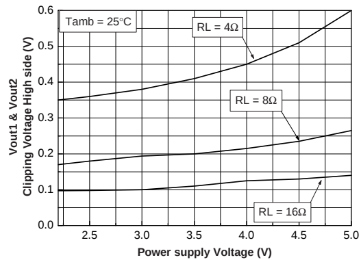
Figure 36. Clipping voltage vs. power supply voltage and load resistor T_{amb} = 25^\circ\text{C}
