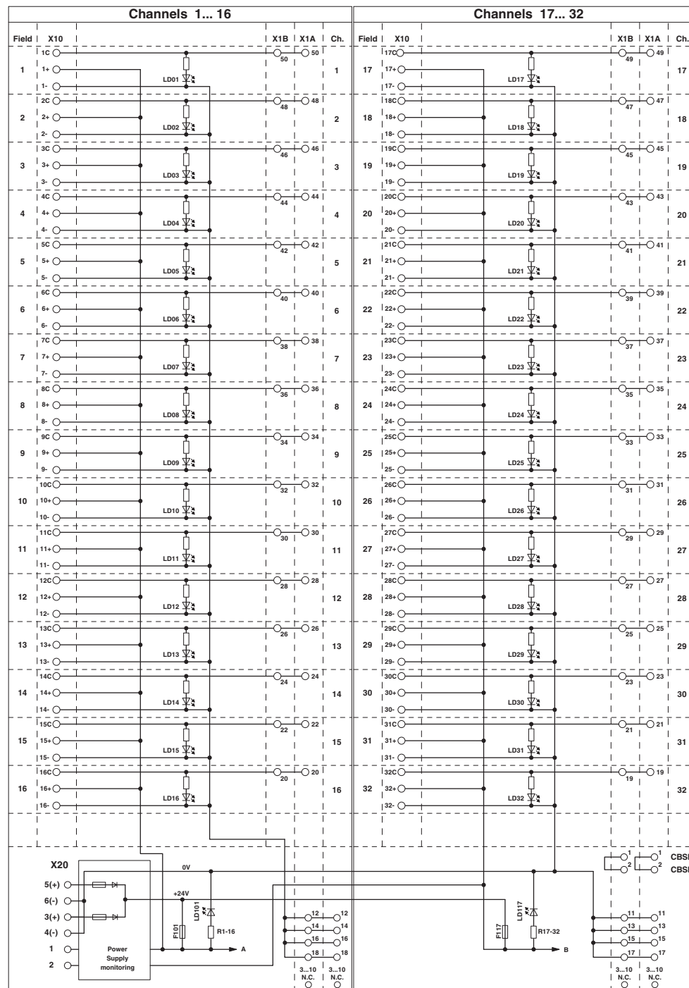
Circuit diagram
