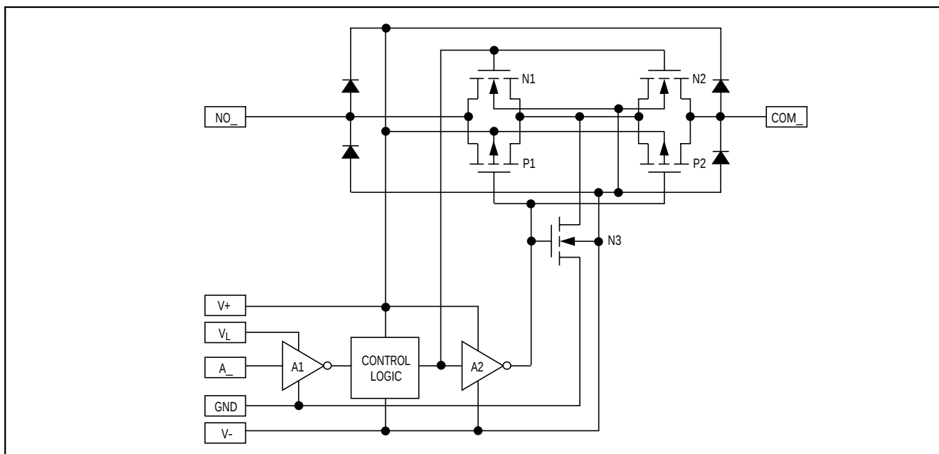
Figure 8. T-Switch Construction
