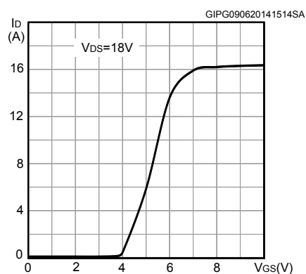
Figure 6. Transfer characteristics
