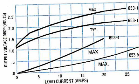
FIGURE 2 - LOAD CURRENT VS. OUTPUT VOLTAGE DROP
