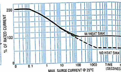
FIGURE 3 - MAX. SURGE CURRENT @ 25°C 653-1, 653-4
