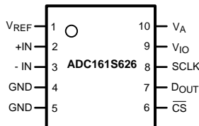
Pin Functions
