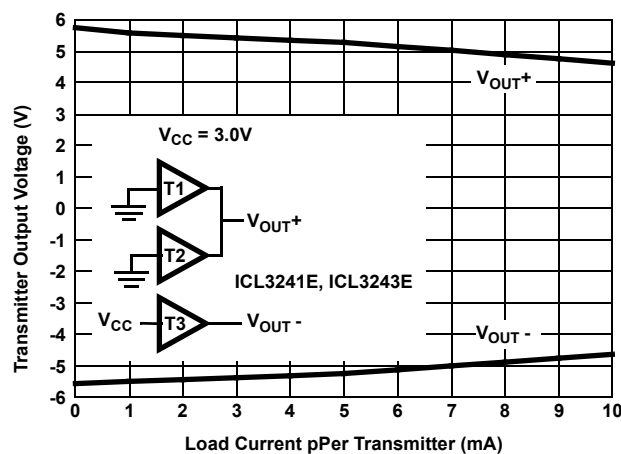
Figure 15. Transmitter Output Voltage vs Load Current (Per Transmitter, Double Current Axis for Total V_{\text{OUT+}} Current)
