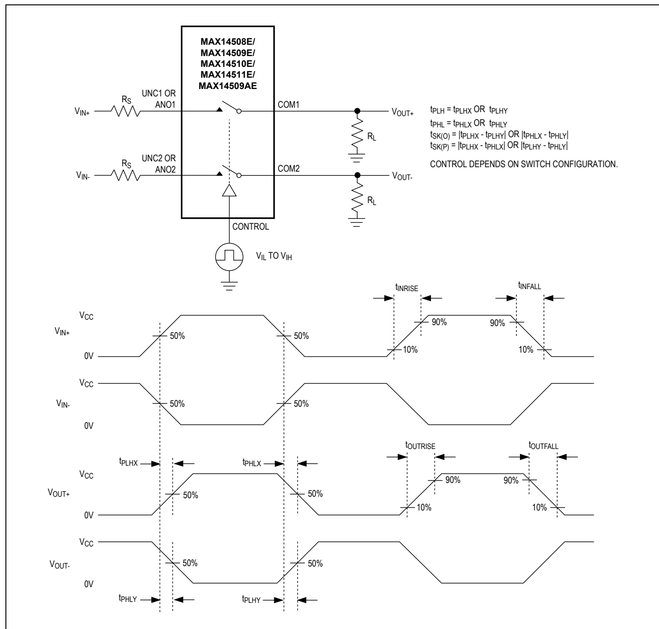
Figure 3. Output Skew
