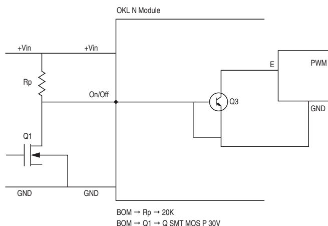
Figure 8. On/Off Circuit Control for Using Negative On/Off Logic
