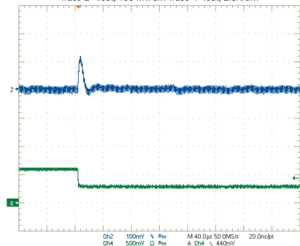
Step Load Transient Response (Vin=12V, Vout=1.2V, Clad=0, Iout=3A to 1.5A) Trace 2=Vout, 100 mV/div. Trace 4=Iout, 2.5A/div.
