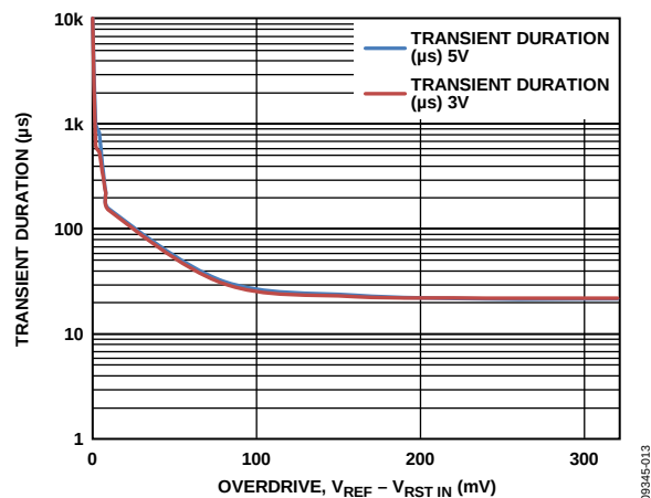
Figure 13. Maximum Transient Duration vs. RST INx ( V_{TH} = 0.4\text{ V} ) Threshold Overdrive
