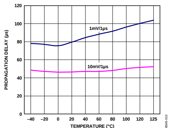
Figure 10. RST IN (V TH = 1.23 V) Falling Propagation Delay vs. Temperature
