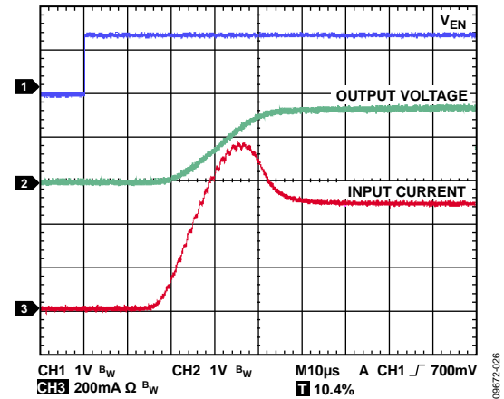
Figure 26. Typical Turn-On Time and Inrush Current, V_{IN} = 1.8V , 500 mA Load, C_{OUT} = 4.7\mu F
