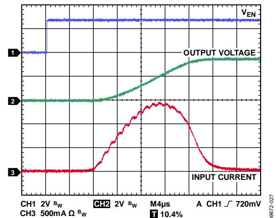
Figure 27. Typical Turn-On Time and Inrush Current, V_{IN} = 3.6V , 10 mA Load, C_{OUT} = 4.7\mu F
