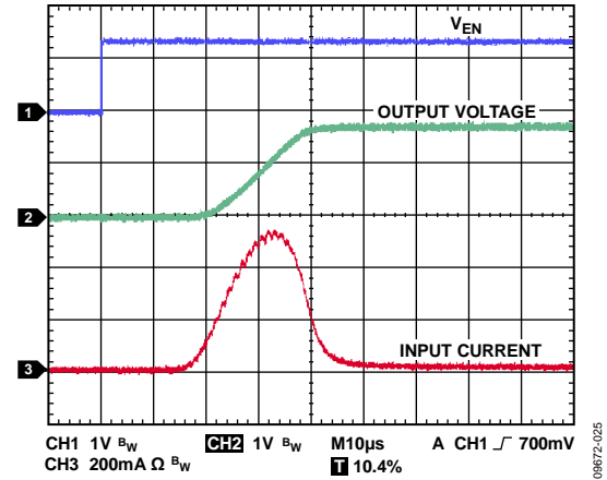
Figure 25. Typical Turn-On Time and Inrush Current, V_{IN} = 1.8V , 10 mA Load, C_{OUT} = 4.7\mu F
