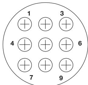
Arrangement 17-9 Max. Wire Ins. Dia. = .150 [3.81]
