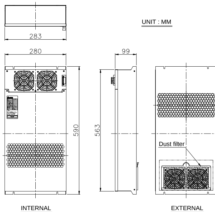
Dimension drawing
