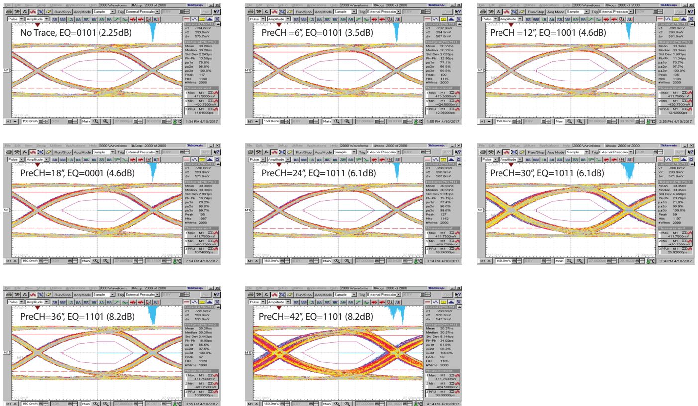
Figure 2-1: Pre-channel length/insertion loss and EQ compensation
