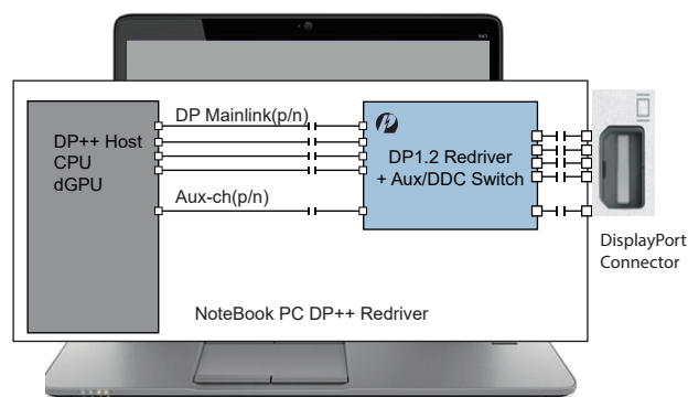
Figure: NB Application Block Diagram
