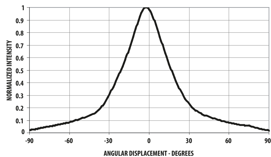
Figure 9: Radiation Pattern
