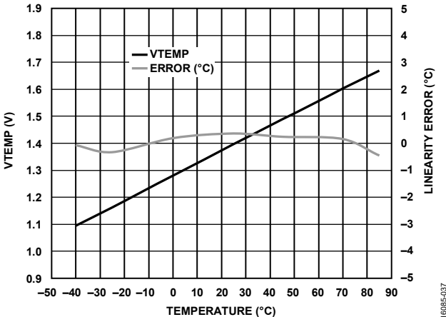
Figure 35. V_{\text{TEMP}} and Linearity Error vs. Temperature
