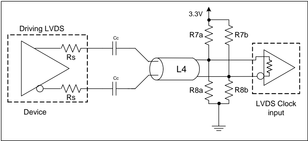
Driving LVDS inputs
