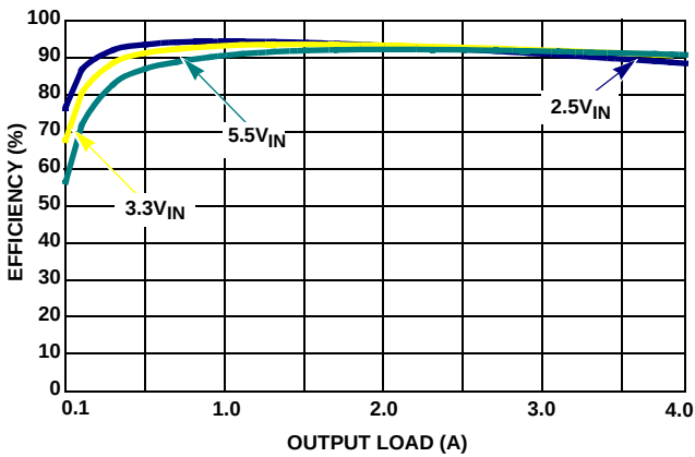
FIGURE 6. V_{OUT1} = 1.8V EFFICIENCY vs LOAD
