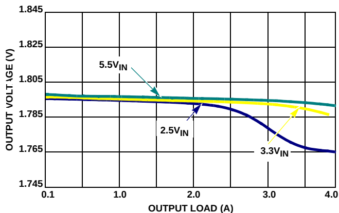
FIGURE 14. V_{OUT1} = 1.8V REGULATION vs LOAD
