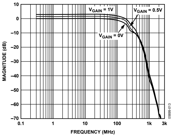
Figure 6. Frequency Response for Various V GAIN Settings Without Cable
