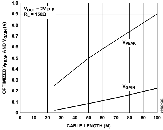
Figure 4. V PEAK and V GAIN Settings vs. Cable Length
