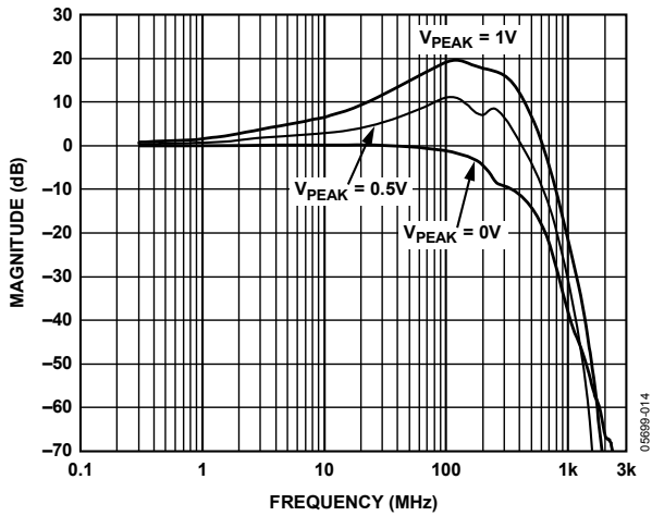
Figure 5. Frequency Response for Various V PEAK Settings Without Cable
