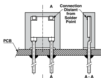
FIGURE 7 – IMPROVED STABILITY WITH THROUGH-HOLE
