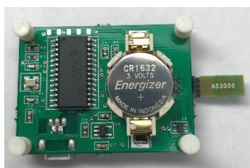
Figure 5. Battery Installation
