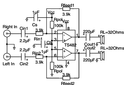
Typical application schematic
