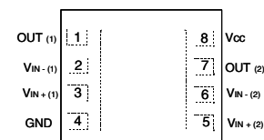
TS482IQT - DFN8
