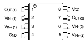
TS482IQT - DFN8
