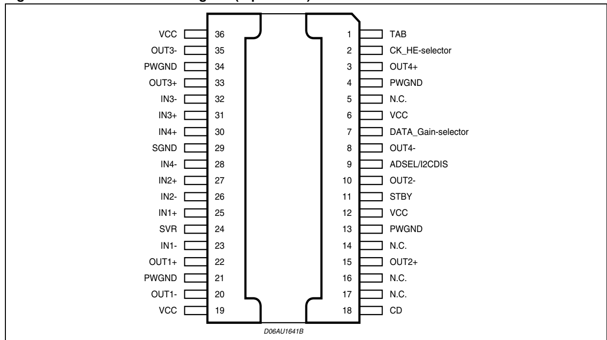
Figure 3. Pins connection diagram (top of view)
