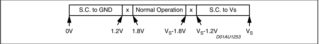
Figure 8. Short circuit detection thresholds
