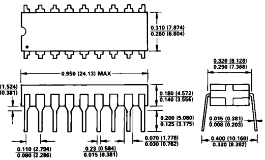
18-Pin Cerdip (Suffix Q)
