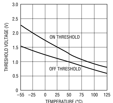
ON/OFF Thresholds
