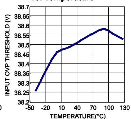
Input OVP Threshold vs. Temperature
