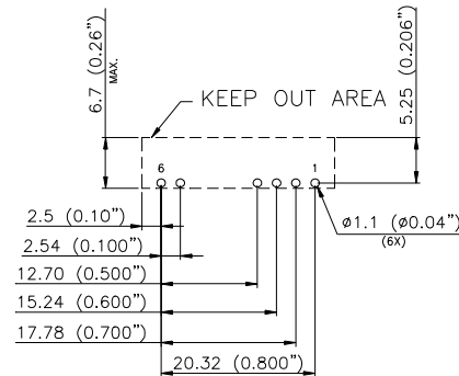
RECOMMENDED PWB PAD LAYOUT
