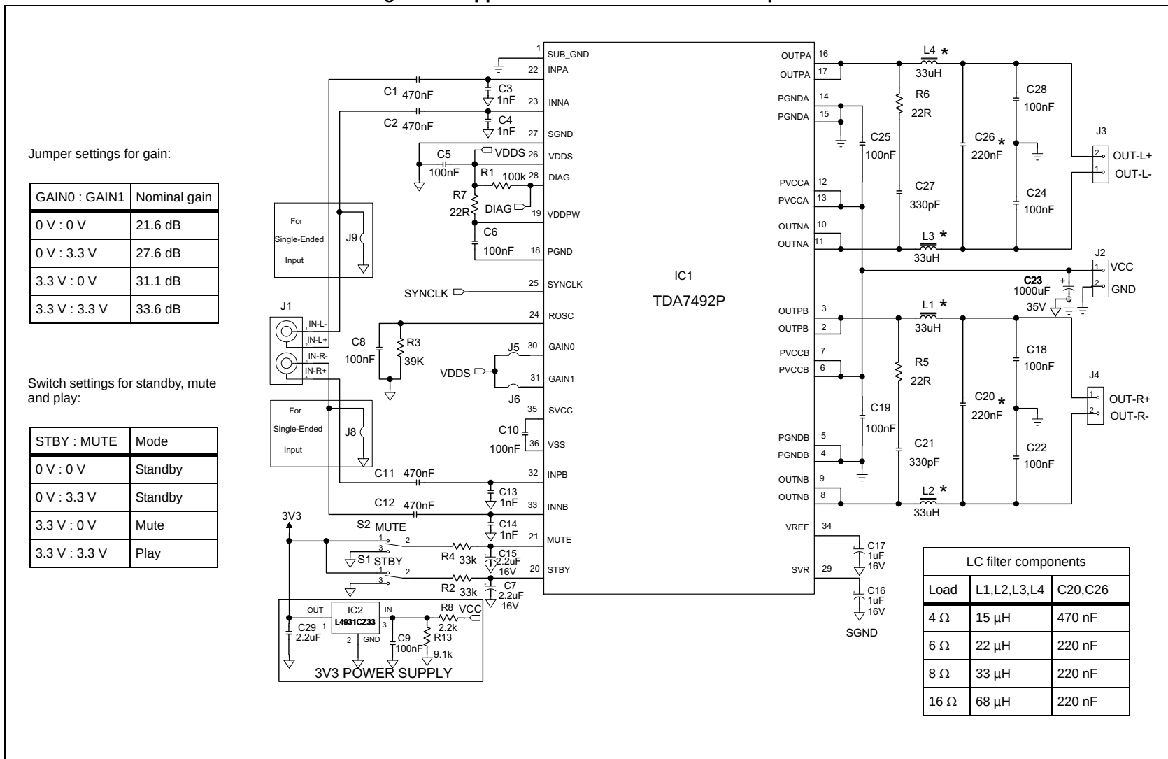
Figure 20. Applications circuit for class-D amplifier
