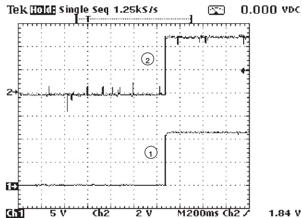
Figure 22 PF/DC OK signal 'V' V1 switch on full load
