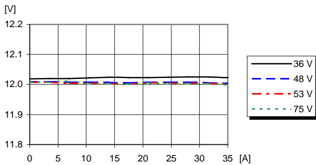
Output voltage vs. load current at T_{P1}, T_{P3} = +25^{\circ}\text{C}
