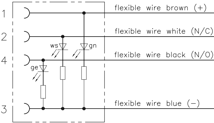
Schematic diagram
