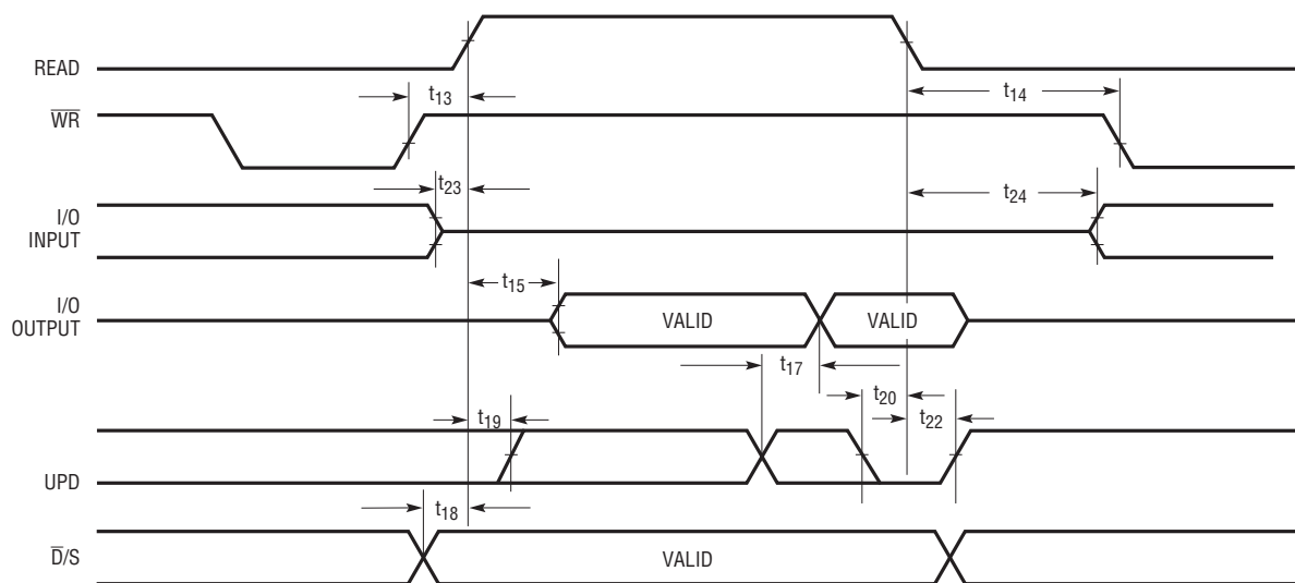
Readback Timing
