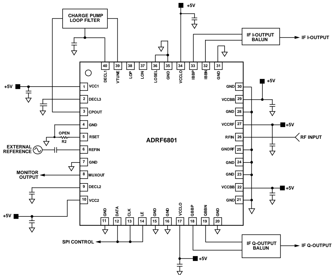
Figure 40. Basic Connections
