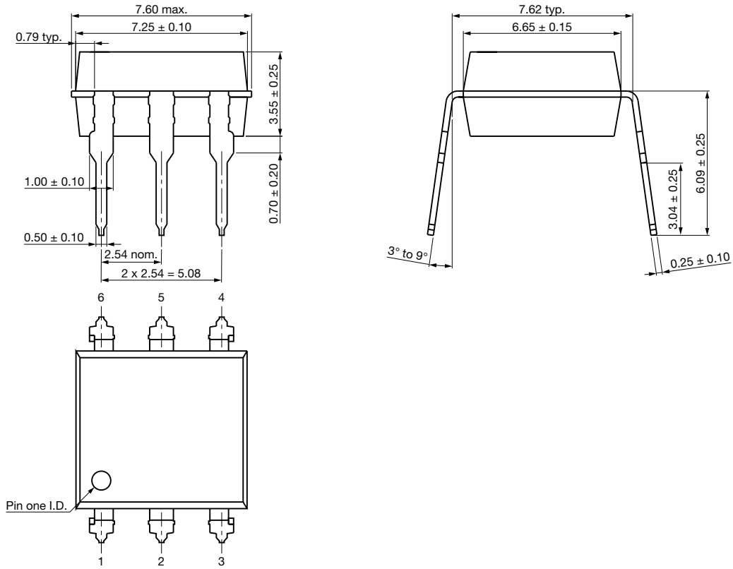
Fig. 16 - Package Drawings
