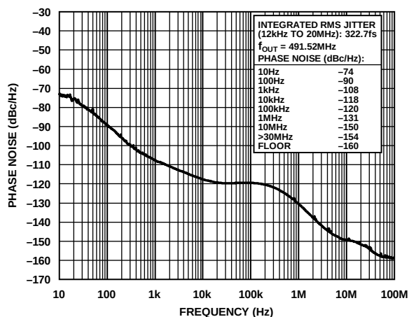
Figure 11. Absolute Phase Noise (PLL1, Configuration 3, HCSSL Mode, f_{REF} = 1\text{ Hz} , f_{OUT} = 491.52\text{ MHz} , f_{COMP} = 19.2\text{ MHz} TCXO, f_{SYS} = 52\text{ MHz} Crystal, BW_{DPLL} = 50\text{ MHz} )
