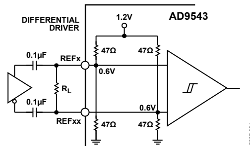
Figure 29. Differential AC-Coupled Mode ( R_1 = 100 \Omega Is Recommended, Except For HCSL)
