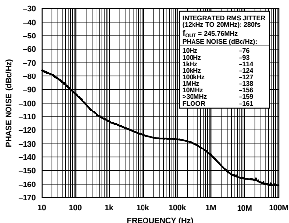
Figure 10. Absolute Phase Noise (PLL1, Configuration 2, HCSSL Mode, f_{REF} = 30.72\text{ MHz} , f_{OUT} = 245.76\text{ MHz} , f_{SYS} = 52\text{ MHz} Crystal, BW_{DPLL} = 50\text{ Hz} )
