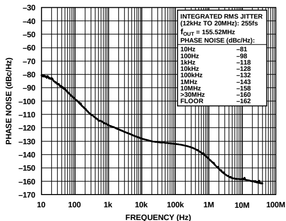
Figure 9. Absolute Phase Noise (PLL1, Configuration 1, HCSSL Mode, f_{REF} = 38.88\text{ MHz} , f_{OUT} = 155.52\text{ MHz} , f_{SYS} = 52\text{ MHz} Crystal, BW_{DPLL} = 50\text{ Hz} )
