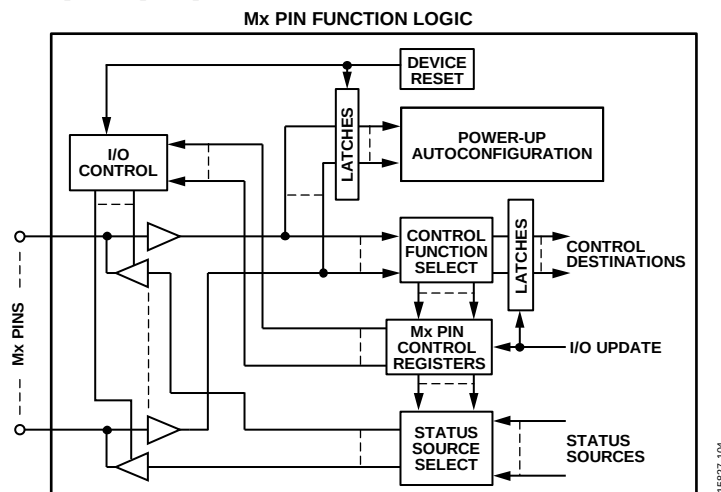
Figure 47. Mx Pin Function Logic
