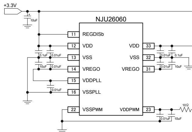
Fig.4 Simple power filter sample
