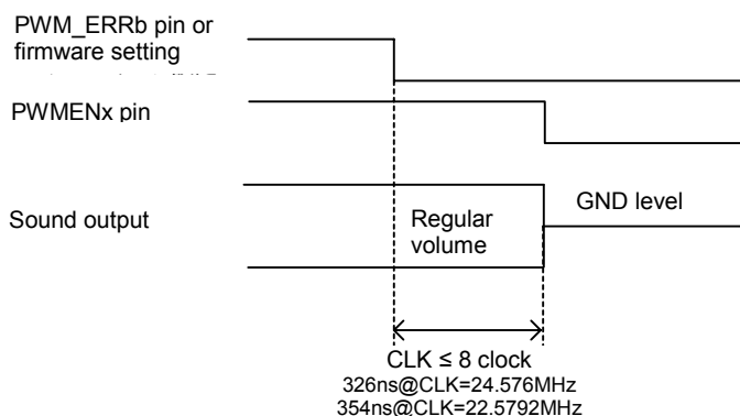
Fig.12 Relation between PWM Reset and PWMEN, PWM Output
