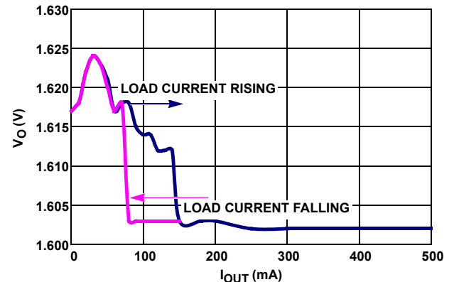
FIGURE 6. OUTPUT VOLTAGE vs LOAD CURRENT ( V_{IN} = 3.6\text{V} , V_{OUT} = 1.6\text{V} )
