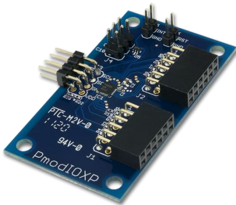
The PmodIEXP.
