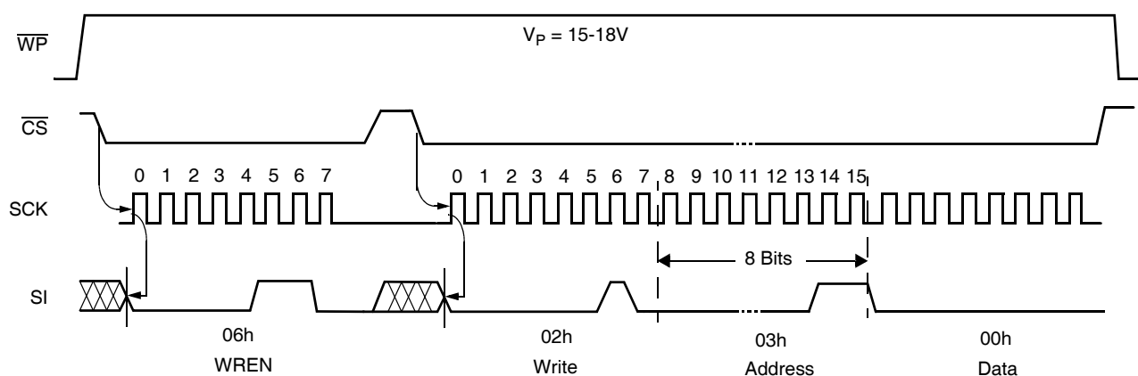
FIGURE 2. RESET V_{TRIP} LEVEL SEQUENCE ( V_{CC} > 3V , \overline{WP} = 15\text{--}18V )
