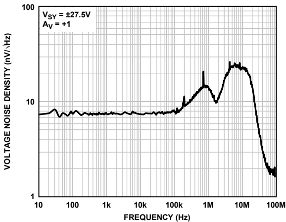
Figure 60. Voltage Noise Density, V_{SY} = \pm 27.5 V
