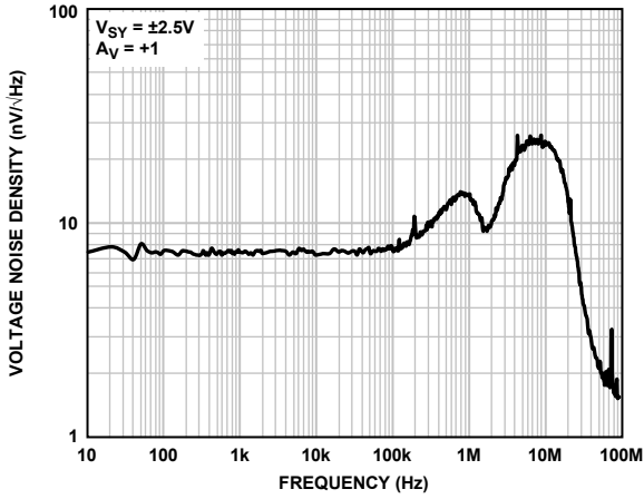
Figure 58. Voltage Noise Density, V_{SY} = \pm 2.5 V
