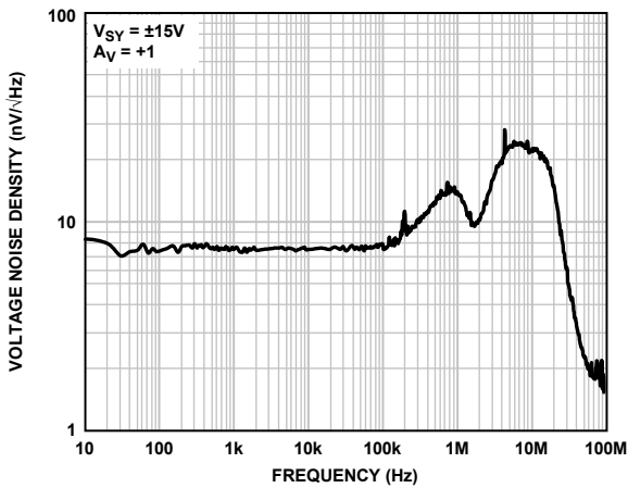
Figure 59. Voltage Noise Density, V_{SY} = \pm 15 V
