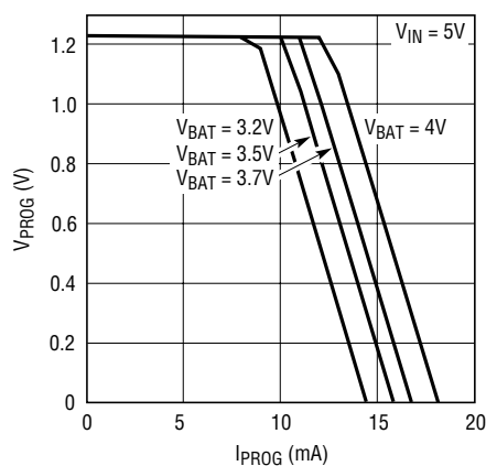
PROG Pin Characteristic (V PROG vs I PROG )
